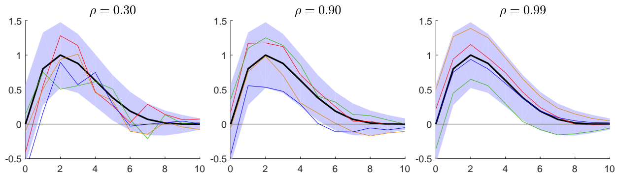
Figure 4: Prior draws of the IRF of the FFR to a demand shock in the bivariate example in Figure 1, for different prior smoothness parameters \rho_{12} . Brightly colored lines are four draws from the multivariate Gaussian prior distribution (7), with the mean and variance parameters in the top right panel of Figure 3 and \rho_{12} \in \{0.3, 0.9, 0.99\} .
