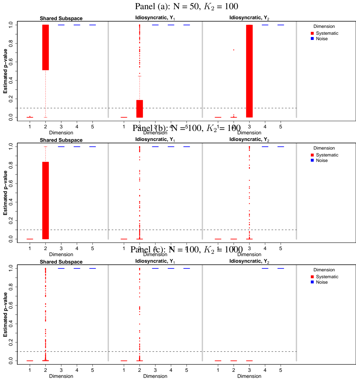
Figure 3: Estimating Dimensions. The three panels above present the results from the permutation test for the number of dimensions under three different settings. We use the same data generation process described in section 4, fixing K_1 = 40 . For panel (a), N = 50 and K_2 = 100 ; for panel (b), N = 100 and K_2 = 100 ; and for panel (c), N = 100 and K_2 = 1000 . Values in the boxplot that fall below the dotted line at p = 0.10 were estimated as systematic dimensions; those above were considered noise. As the three panels show, as we increase both the number of observations N and the number of features ( K_2 ) of the larger data set, MD2S is able to detect the correct dimensionality. Note that for each of the 500 simulations per setting, 500 permuted datasets were used to recover a p -value.
